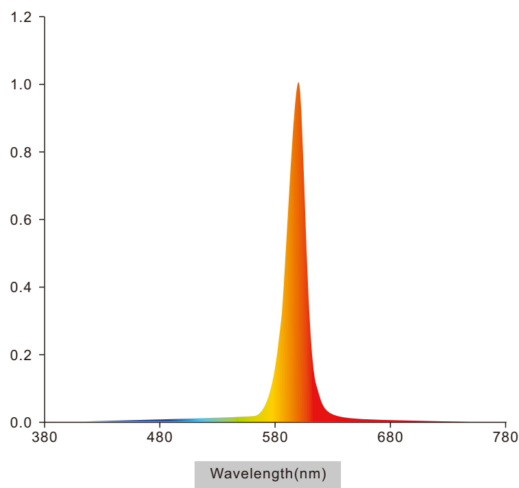
Relative Spectrum
